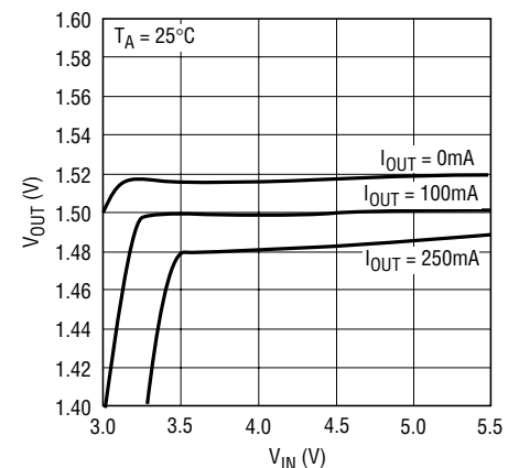
Output Voltage vs Supply Voltage
